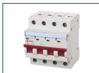
MCB 4P 16A 3kA Type B
