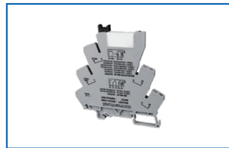
Slim Relay 1co
